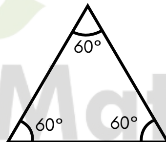
Acute angled Triangle
