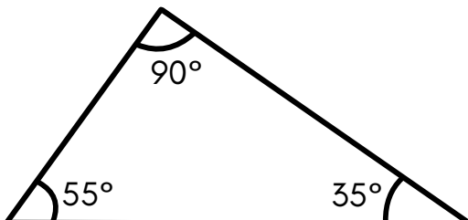
Right angled Triangle
