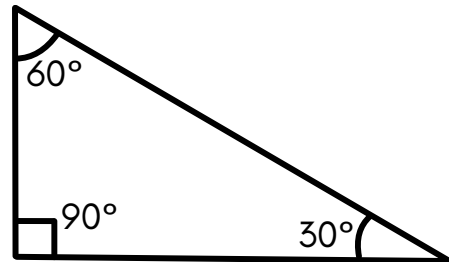
Right angled Triangle
