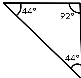
Obtuse angled Triangle
