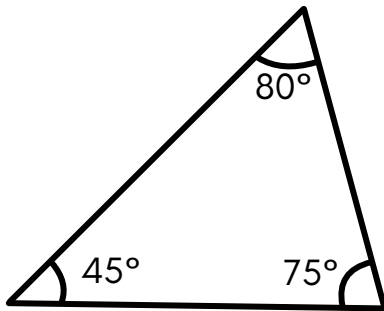
Acute angled Triangle
