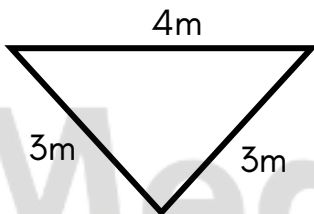
Isosceles Triangle
