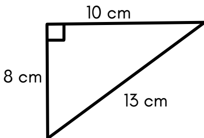
Scalene Triangle
