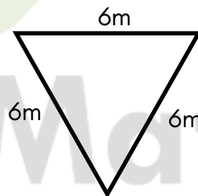
Equilateral triangle
